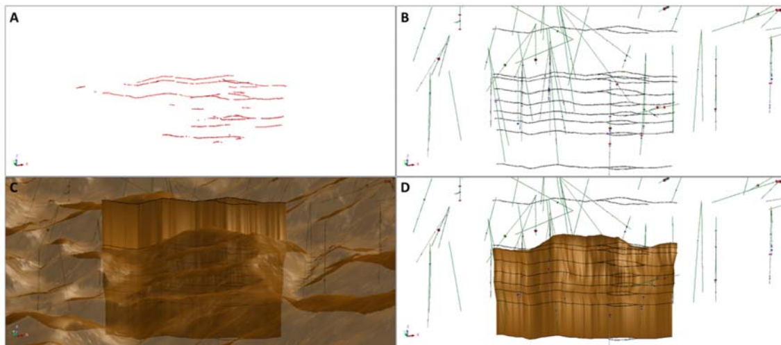
Figure 15.2.2.2: Vein Modelling Procedure: (A) UG channel samples used for modelling loaded in 3D (B) Interpreted vein outlines projected based on the structural interpretation and drill hole data (C) Vein solid rendered from the interpreted sections to be clipped using the surface DTM (D) Final vein solid
