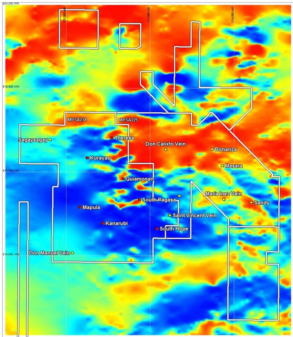
Figure 14.6.5.2.1: TMI (Total Magnetic Intensity) Map
