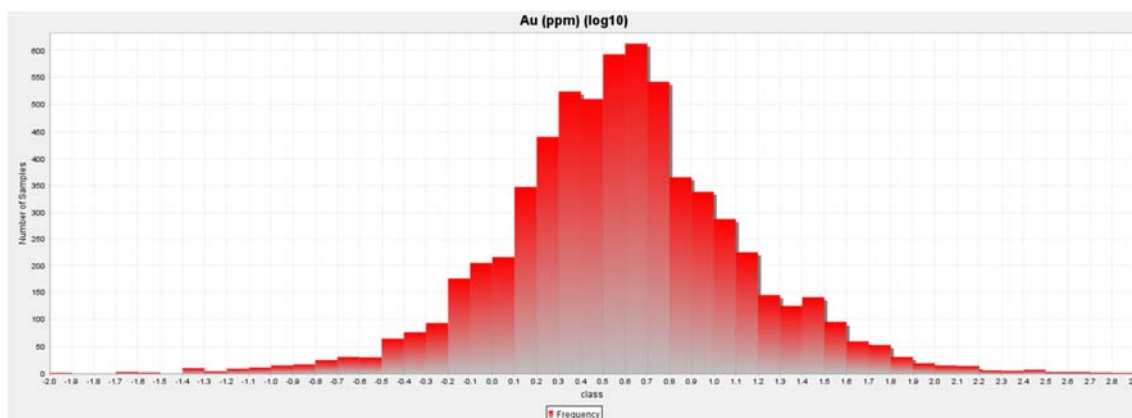
Figure 15.1.3.2.2: Log-transformed Au Grade Histogram of All Samples
