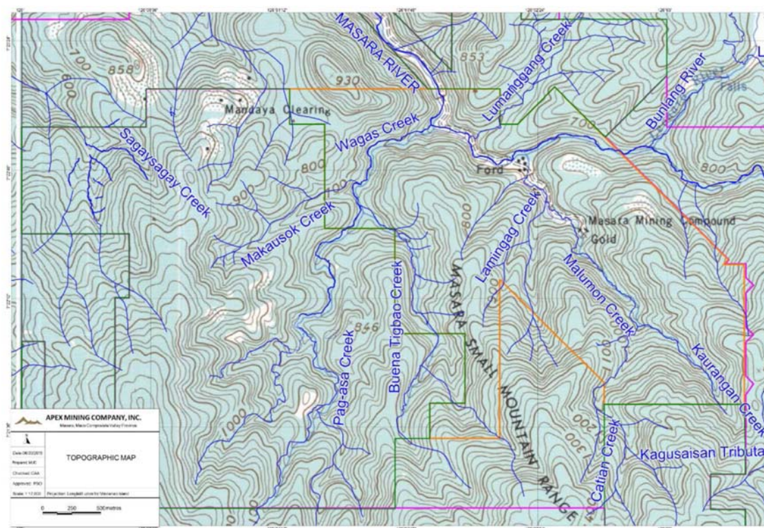
Figure 8.2.1: Topographic Map Showing the Tributaries in the Contract Area
