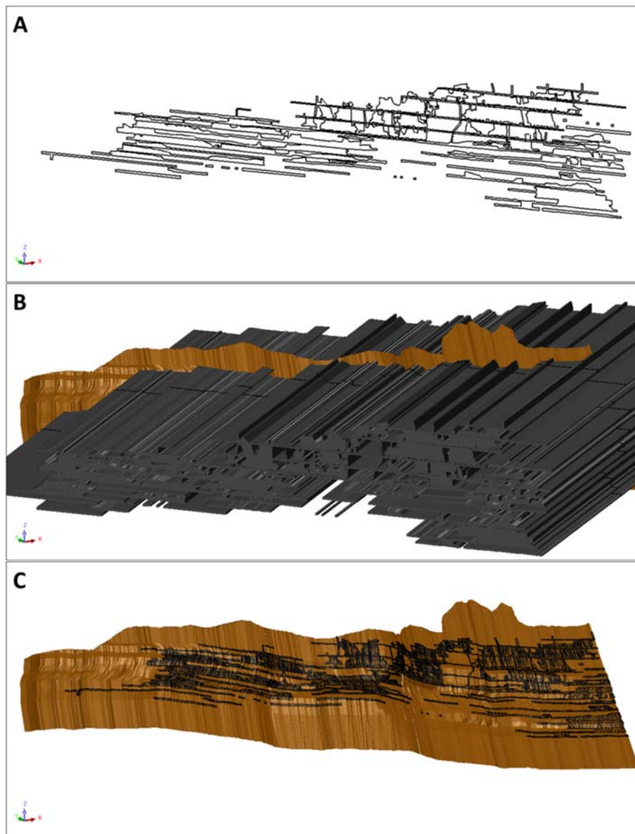
Figure 15.2.3.1: Mined Out Modelling Procedure: (A) Outlines of the mined out portions loaded onto the cutting plane in 3D (B) Solids extruded from the outlines to be intersected with the MV, HW, and FW solids (C) Mined out solid models
